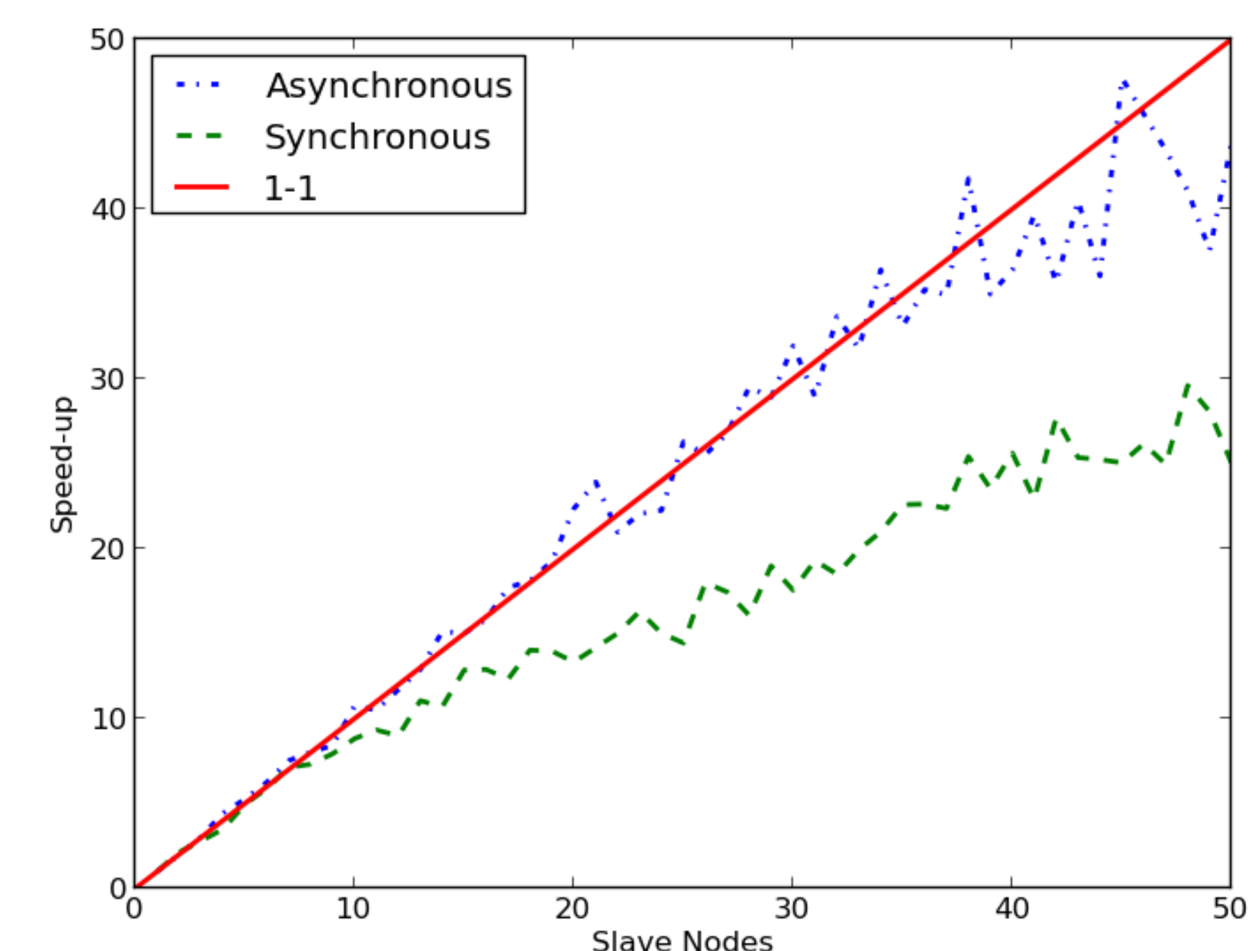
Figure 4: Plot of speed-up of convergence time vs number of slave nodes
