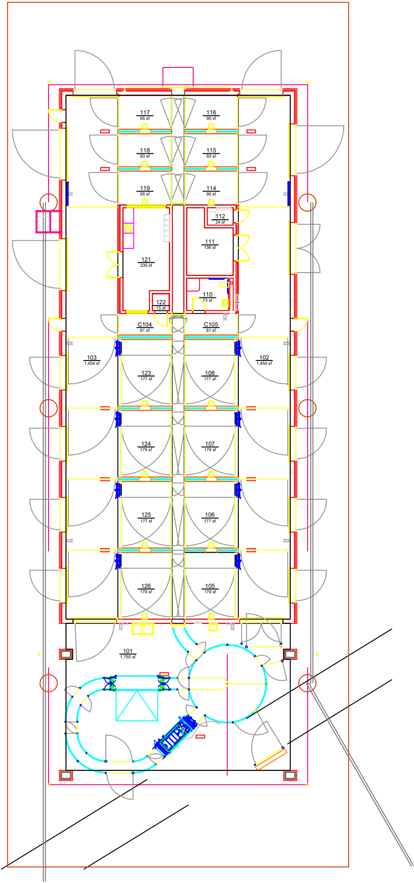
BASE FLOOR PLAN FOOD ANIMAL RESEARCH FACILITY LEVEL: 01
