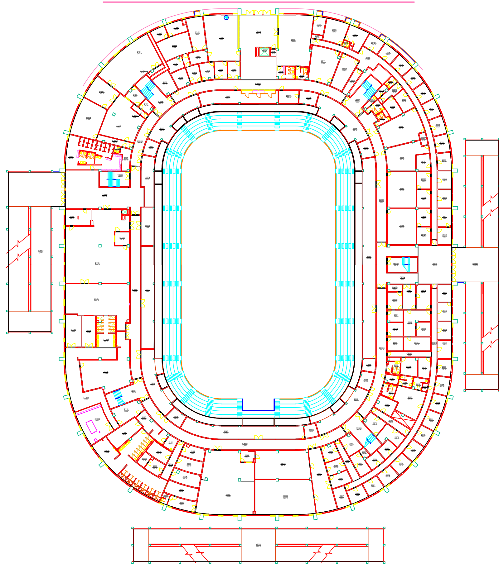
BASE FLOOR PLAN BEARD-EAVES-MEMORIAL COLISEUM LEVEL: 02
