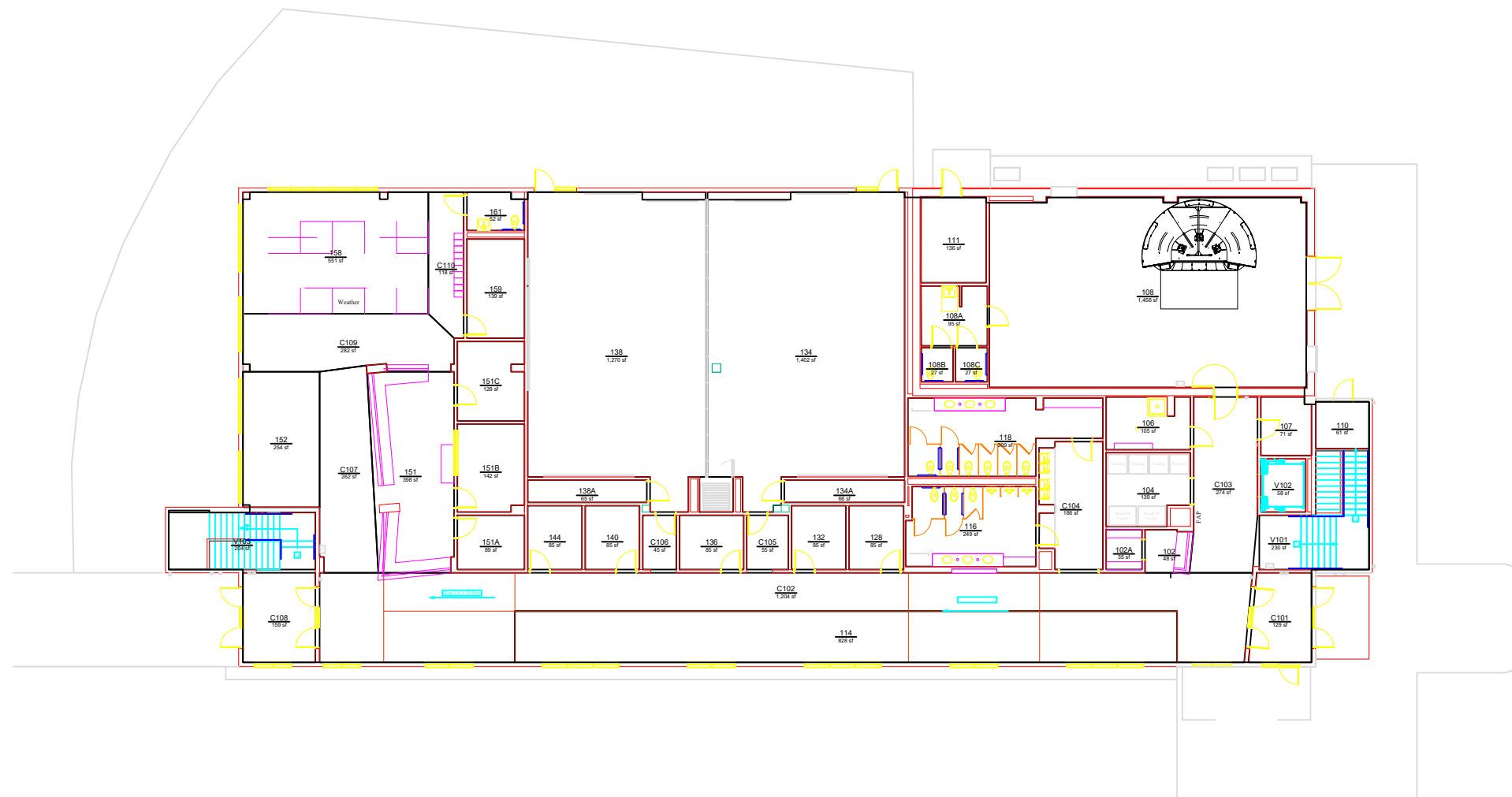
BASE FLOOR PLAN AVIATION EDUCATION: DELTA AIR LINES AVIATION EDUCATION BUILDING LEVEL: 01
