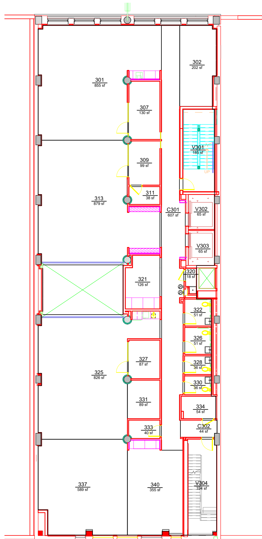
BASE FLOOR PLAN AUBURN IN BIRMINGHAM BUILDING LEVEL: 03
