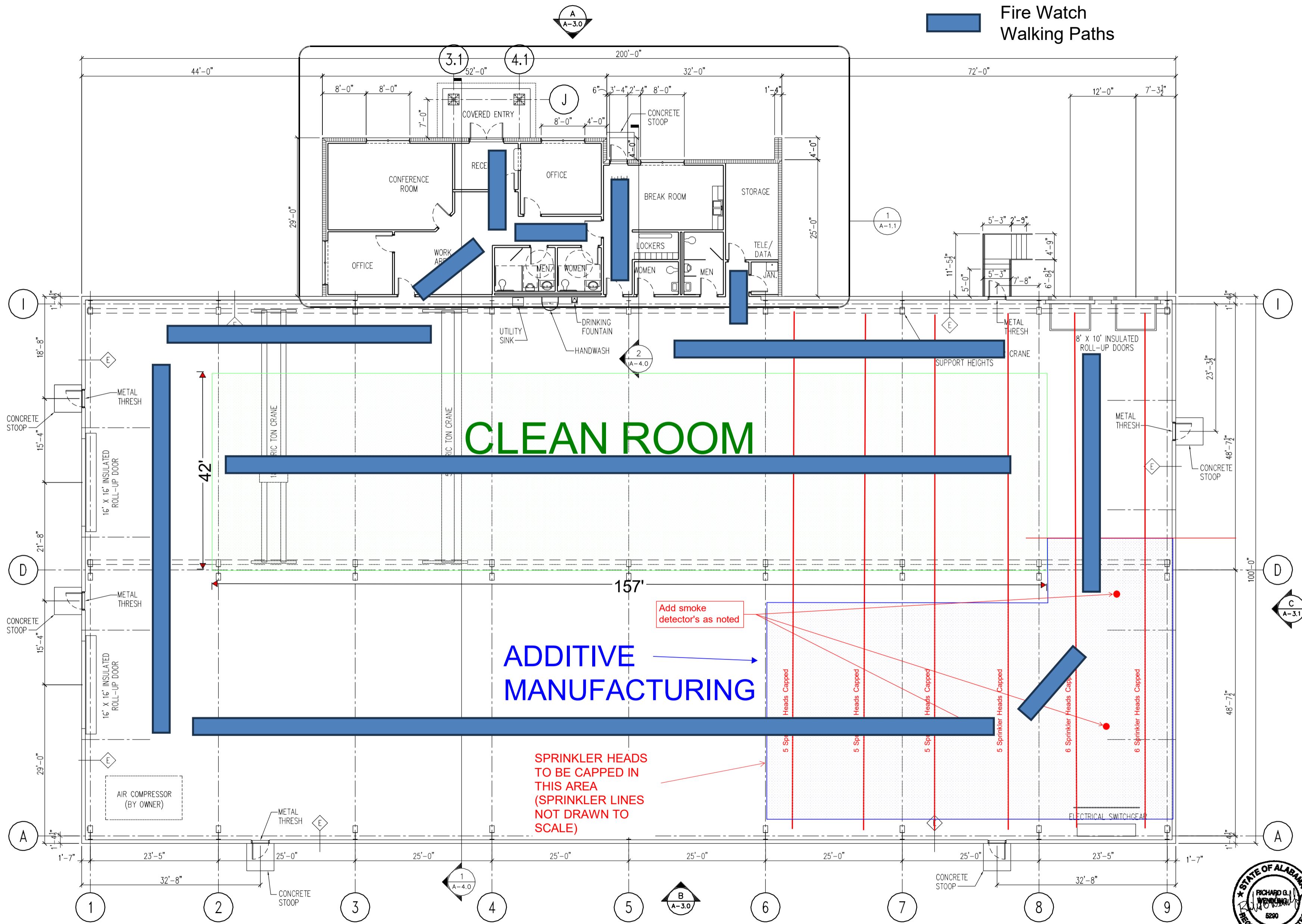
1 OVERALL FLOOR PLAN A-1.0 SCALE: 1/8" = 1'-0"
